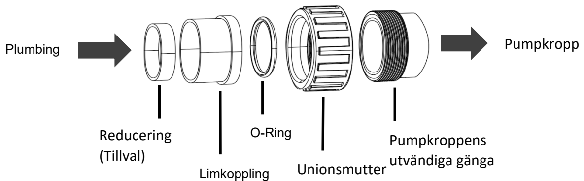
Figur 3 – Union Kit
